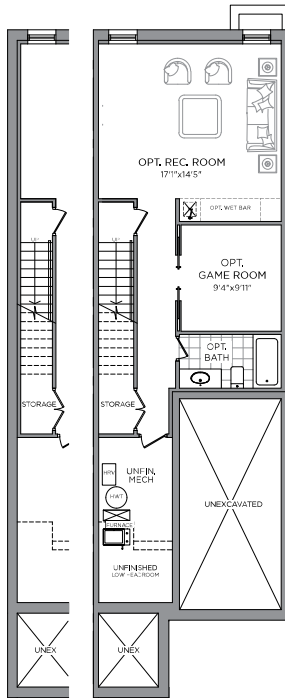
END OPT. BASEMENT FLOOR PLAN FINISHED REC ROOM
