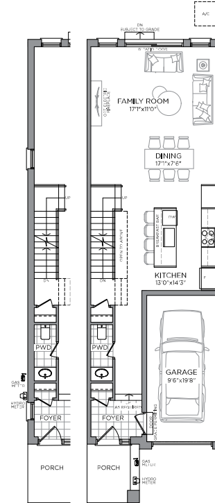
END GROUND FLOOR PLAN
