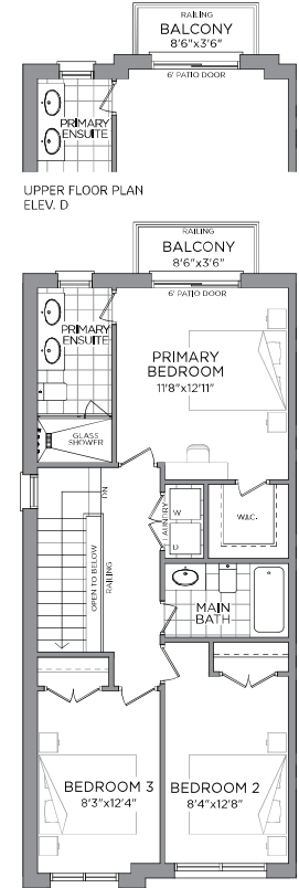
UPPER FLOOR PLAN ELEV. A & B
