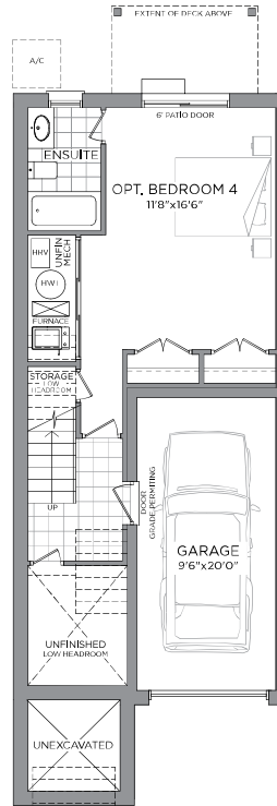
OPT. GROUND FLOOR PLAN ELEV. A & B FINISHED 4TH BEDROOM
