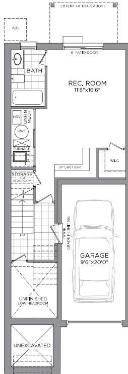
GROUND FLOOR PLAN ELEV. A & B FINISHED SUITE
